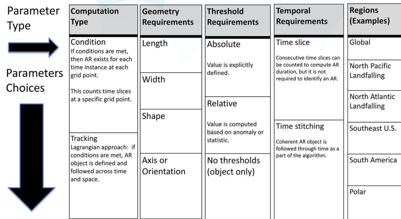
Figure 5. Schematic diagram illustrating the diverse components of AR detection algorithms. Parameter types commonly applied include computation type, geometric moisture threshold, and temporal requirements, as well as algorithms developed for global ARs or specific geometric regions. (Shields et al. 2018.)
