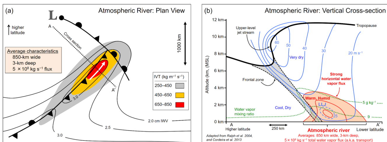
Figure 1. From the AMS Glossary of Meteorology and the result of a consensus-driven effort to define an atmospheric river (a) shows the AR Plan View and (b) shows the vertical cross-section.
