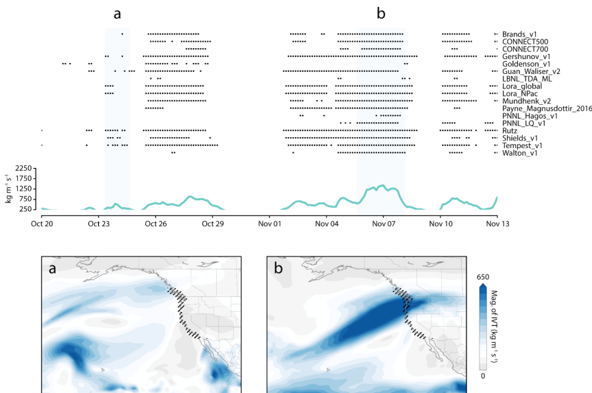
Figure 7. Time series of the magnitude of IVT along the U.S. west coast in teal for October 20 – November 13th 2006. The dots at the top of the figure show time steps with AR conditions along the coastline for each of the algorithms. Two events are highlighted in light blue to show the range of agreement between the algorithms. Panel (a) shows a composite in IVT of a relatively smaller event that was identified in only eight algorithms (averaged between Oct 23 09 UTC and Oct 24 15 UTC) and panel (b) shows a much stronger event captured by nearly all algorithms (averaged between Nov 05 15 UTC and Nov 08 03 UTC). The region used to determine landfall is hatched in both (a) and (b). The first event falls along the northern edge of the landfalling domain and highlights that differences in the spatial extent of the AR id might influence landfall rates.
