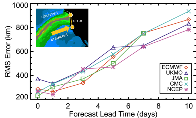
Figure 2. 400-km AR landfall position forecast error at a 3-day lead time. AR forecast skill assessment establishes a performance baseline. (Wick et al. 2013). From “AR Reconnaissance” presentation by F.M. Ralph (Scripps/CW3E).
