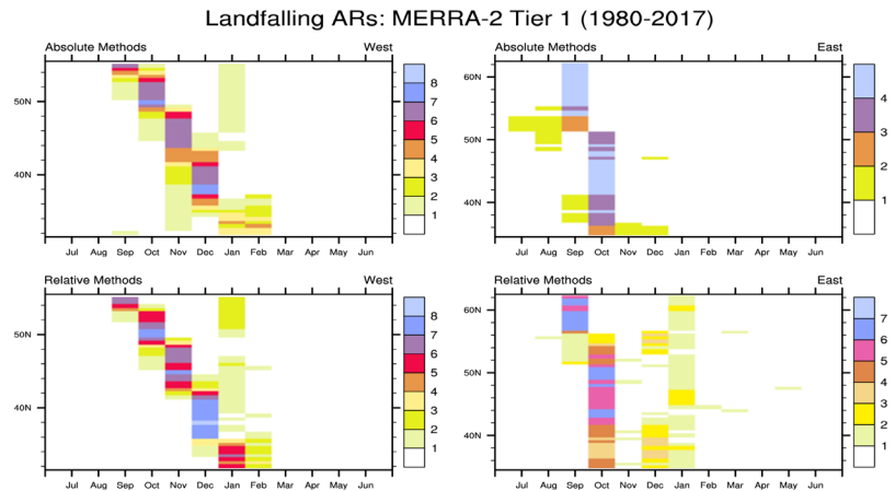
Figure 6. Agreement amongst methodologies for the month of maximum frequency for landfalling ARs. The west coast of North America (West) and Europe (East) are shown. Plotted in color pixels are the number of methods using absolute (relative) moisture thresholds for a given month. The color bar maximum value corresponds to the number of methods possible for this category. For example, for absolute methods applied to Europe (East) (top right panel), the total possible number of methodologies is 4 and is plotted in light blue. All 4 absolute/east methods agree in September as the month with maximum frequency of landfalling ARs for latitudes 55-62N. MERRA-2 for 1980-2017 were used.
