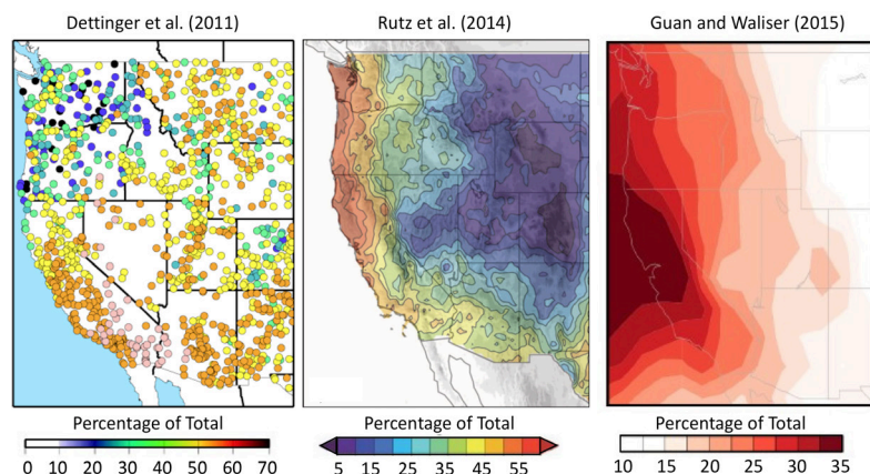
Figure 4. Shown (left and center) is the fraction of cool-season precipitation attributable to ARs from Dettinger et al. (2011) and Rutz et al. (2014). (Right) As in left and center, but for annual precipitation. These studies use different AR identification methods, as well as different atmospheric reanalyses and observed precipitation data sets.
