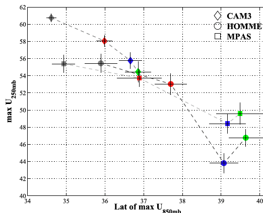
Figure 3. Latitude of the zonal wind maximum at 850 hPa (in degree) and the 250 hPa maximum zonal wind (in m s^{-1} ) in simulations with different dynamical cores and model resolutions. The subtropical jet location and strength are sensitive to resolution with a hint of convergence at \sim 50 km grid spacing (Lu et al. 2015).
